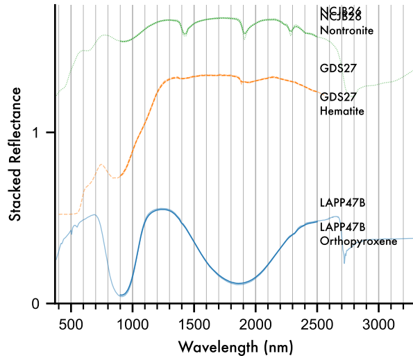
Enfys_Ingaas_Mwir Sampled Lapp47B Orthopyroxene, Ncjb26 Nontronite, Gds27 Hematite grouped by Sample Id with Noise
